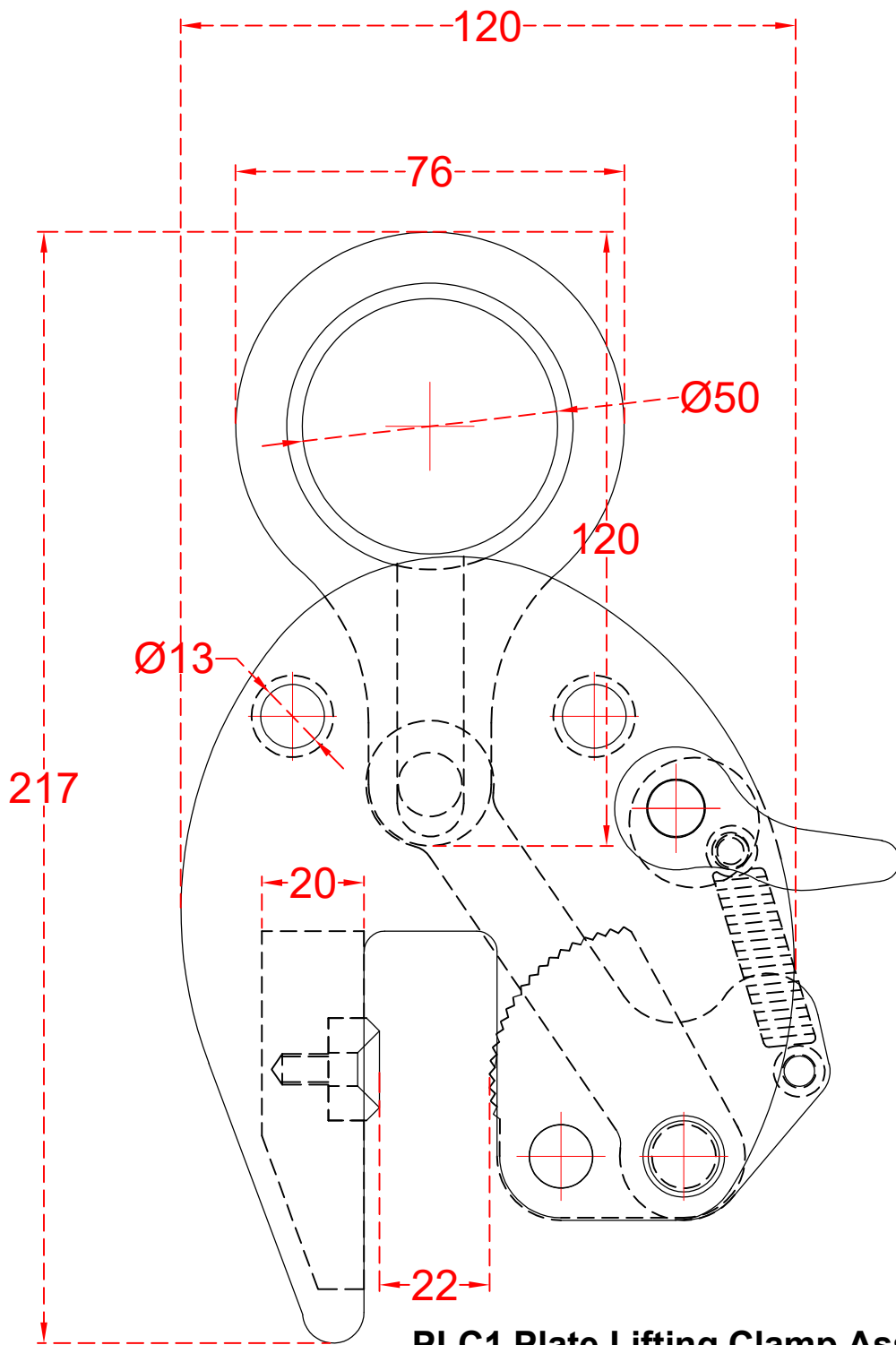
PLC1 Plate Lifting Clamp Assembly 1016kg (1T) WLL 0-20mm Plate Thickness Adjustment 2.5kg Average Weight
